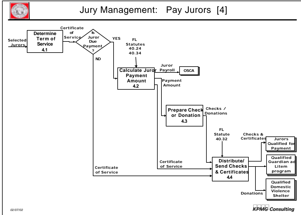
Figure A-43. Pay Jurors [4]
