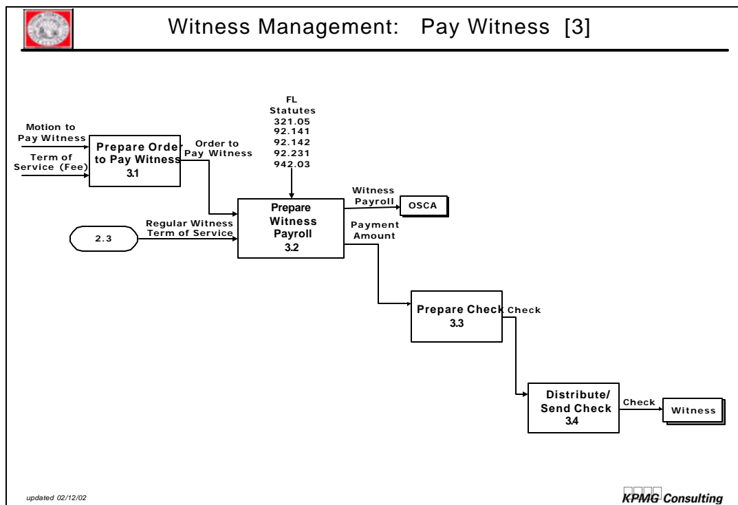
Figure A-48. Pay Witness [3]
