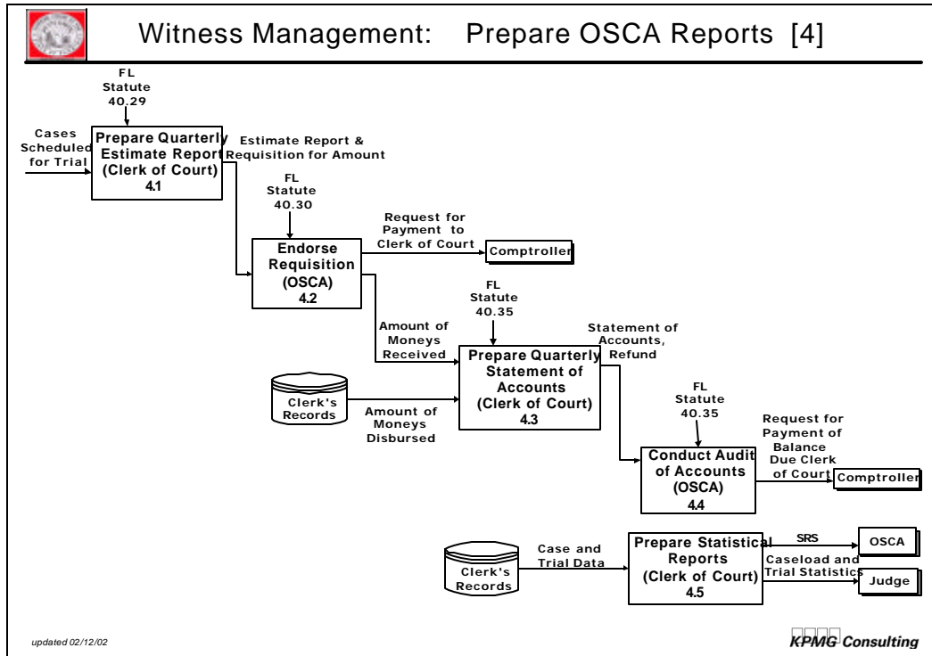
Figure A-49. Prepare OSCA Reports [4]
